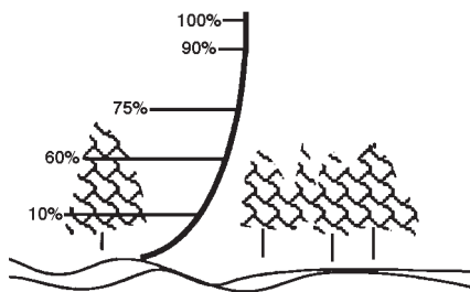
Figure 2. Height Over Rough Terrain Vs. Percentage of Maximum Wind Speed
